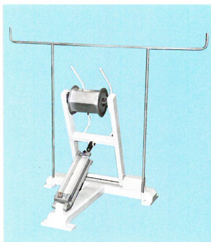
缓冲装置 Buffering device
