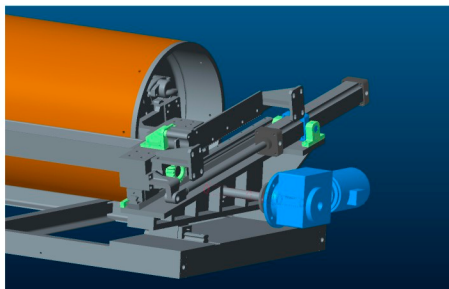
压辊左右微调装置 Fine adjust device on right and left side of press roller
